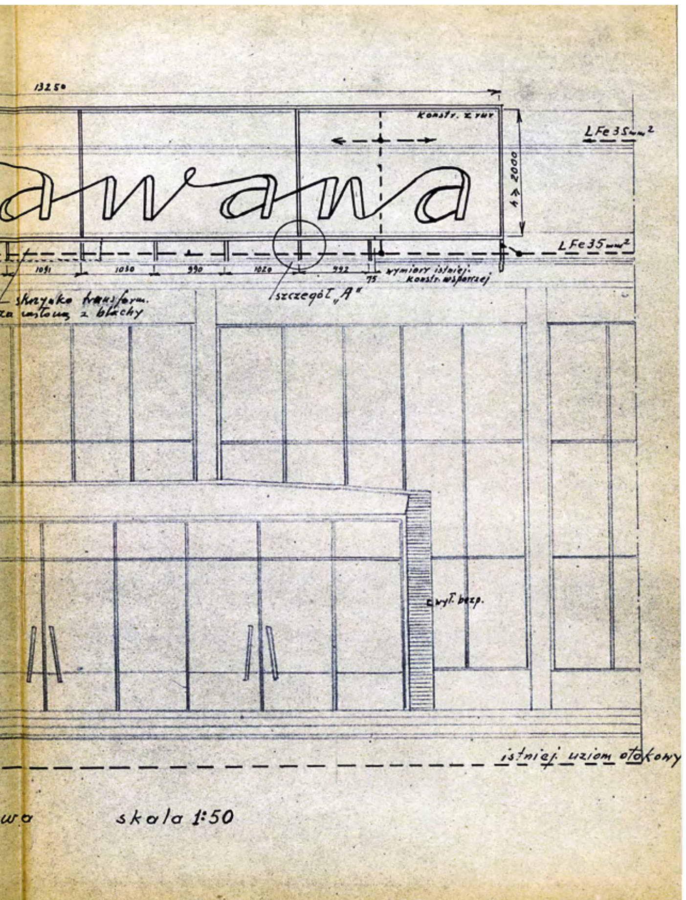
■ Technical documentation of the cinema „Havana”, 1966. Presidium of the Municipal National Council in Piotrków Trybunalski, sig. 1617.
