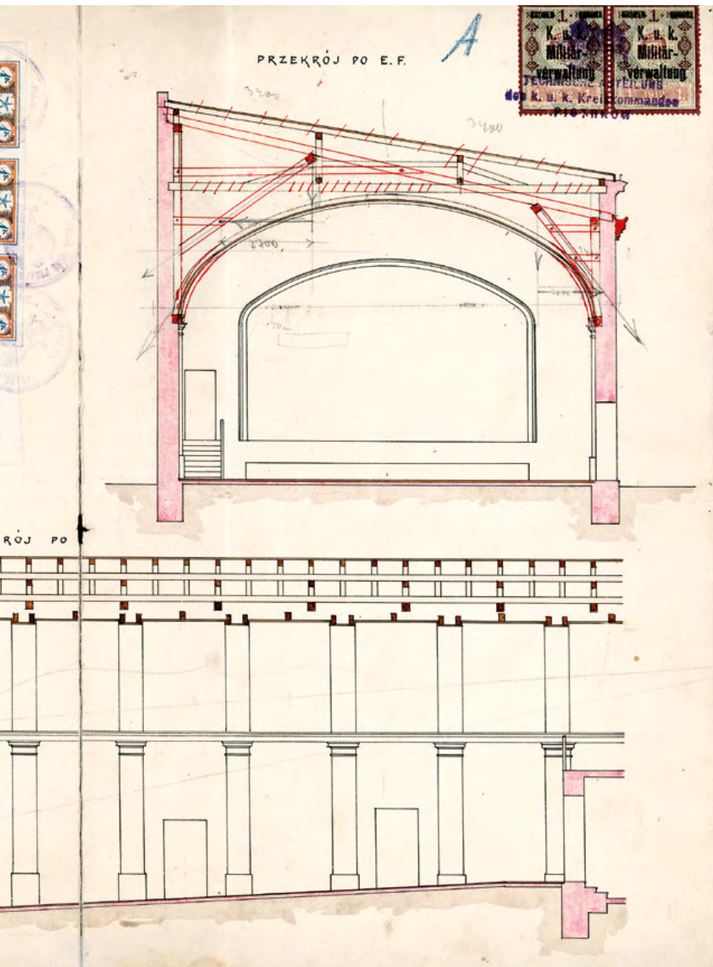
■ The plan of cinema „Czary”, 1917. District office of Piotrków, sig. 138.
